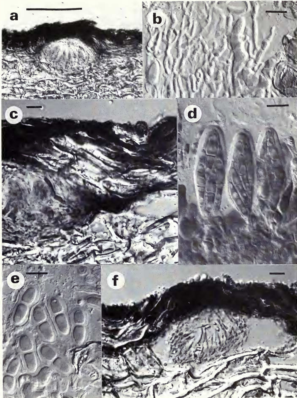
Fig. 27 Arthopyrenia umbripicta Norman (O-holotype). (a) Vertical section of ascoma; scale = 100 \mu\text{m} ; (b) Pseudoparaphyses; (c) Detail of involucrellum showing clypeus; (d) Asci and ascospores; (e) Ascospores; (f) Conidioma and conidia; scale = 10 \mu\text{m} .
